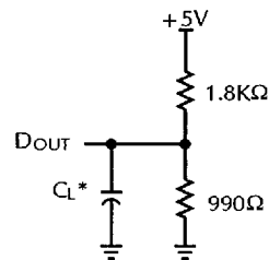
Figure 1. Output Load * Including Scope and Jig Capacitance.
